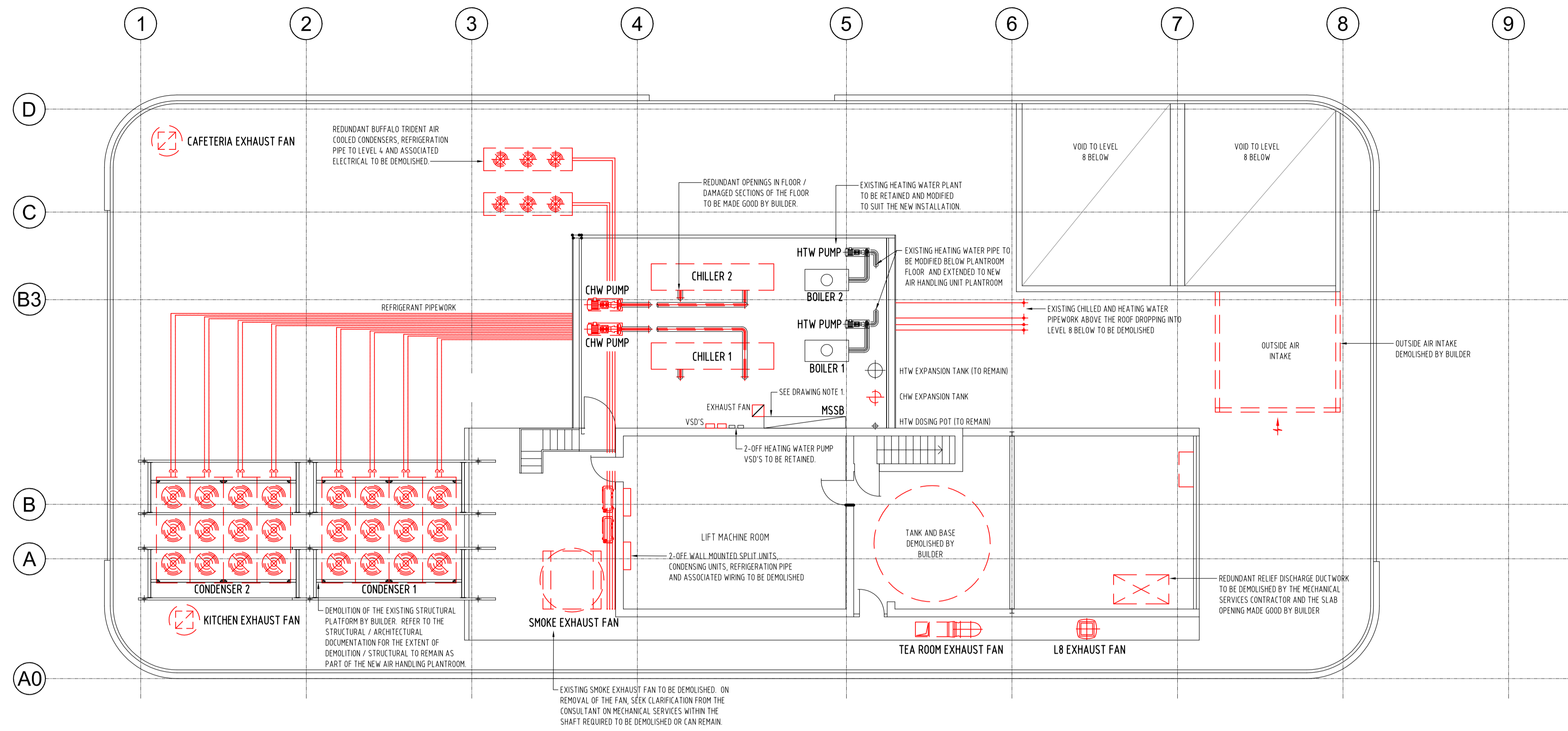
ROOF - MECHANICAL SERVICES DEMOLITION SCALE 1:100
