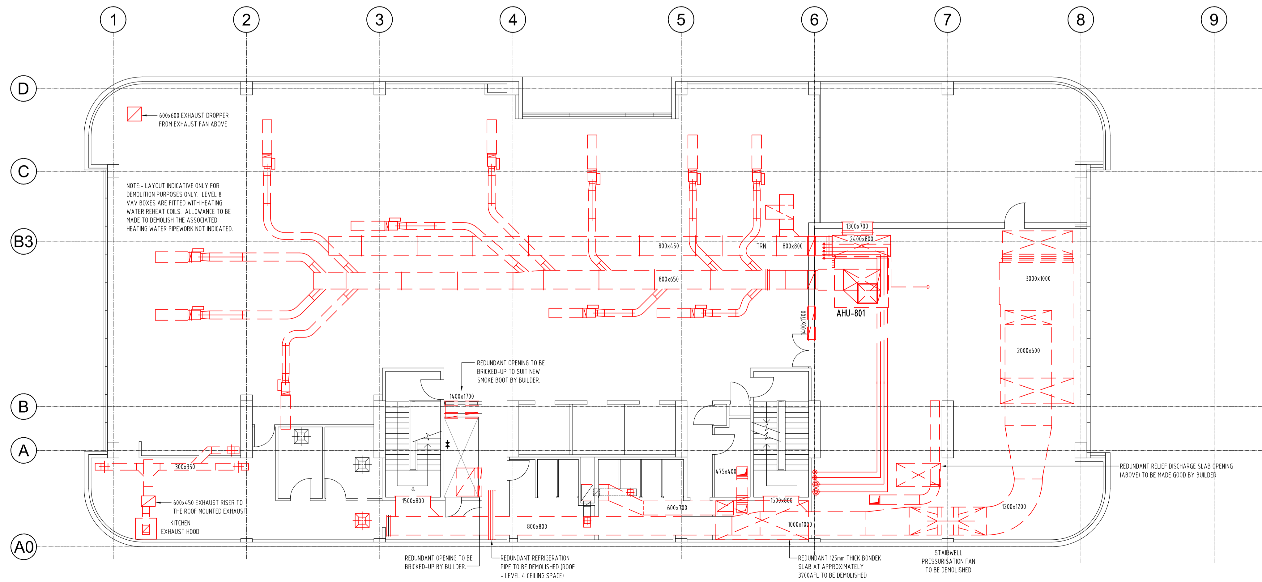
LEVEL 8 - MECHANICAL SERVICES DEMOLITION SCALE 1:100
