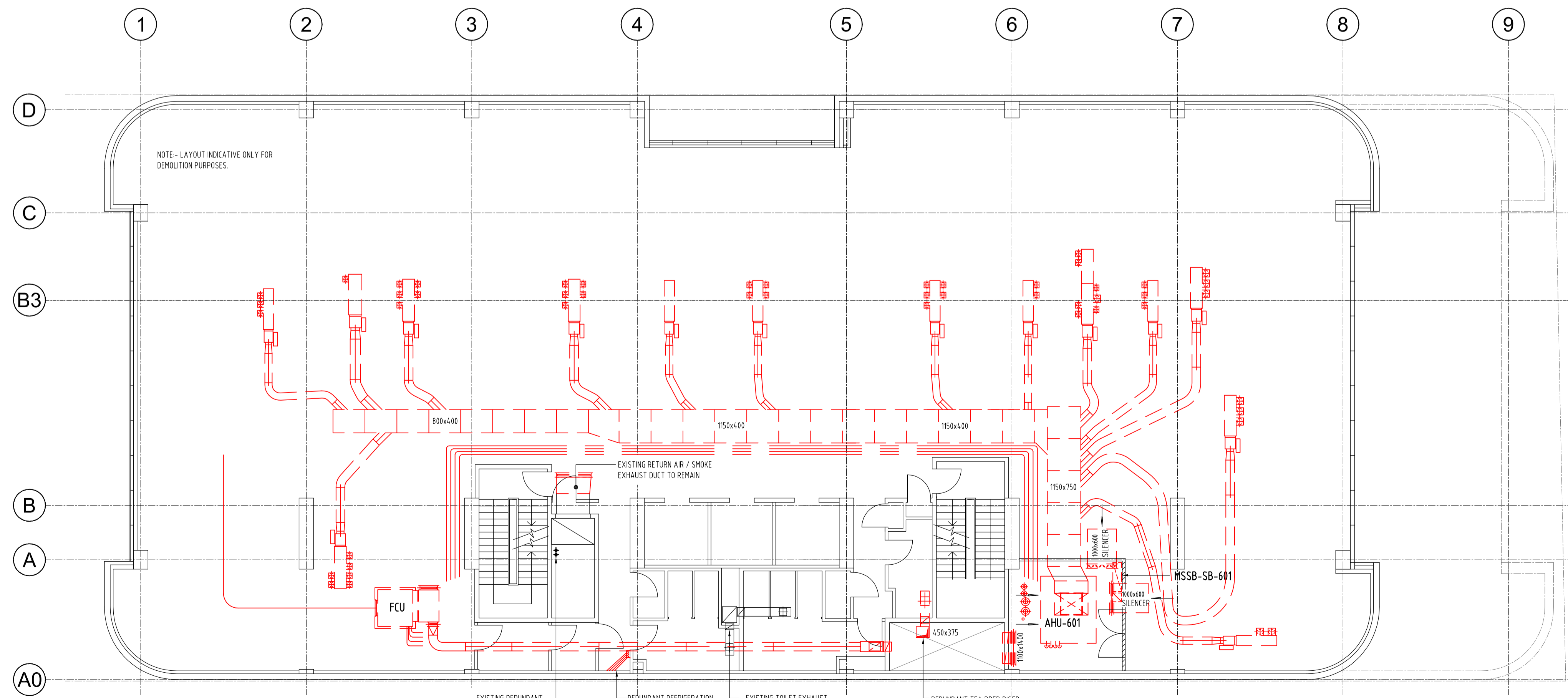
LEVEL 6 - MECHANICAL SERVICES DEMOLITION SCALE 1:100
