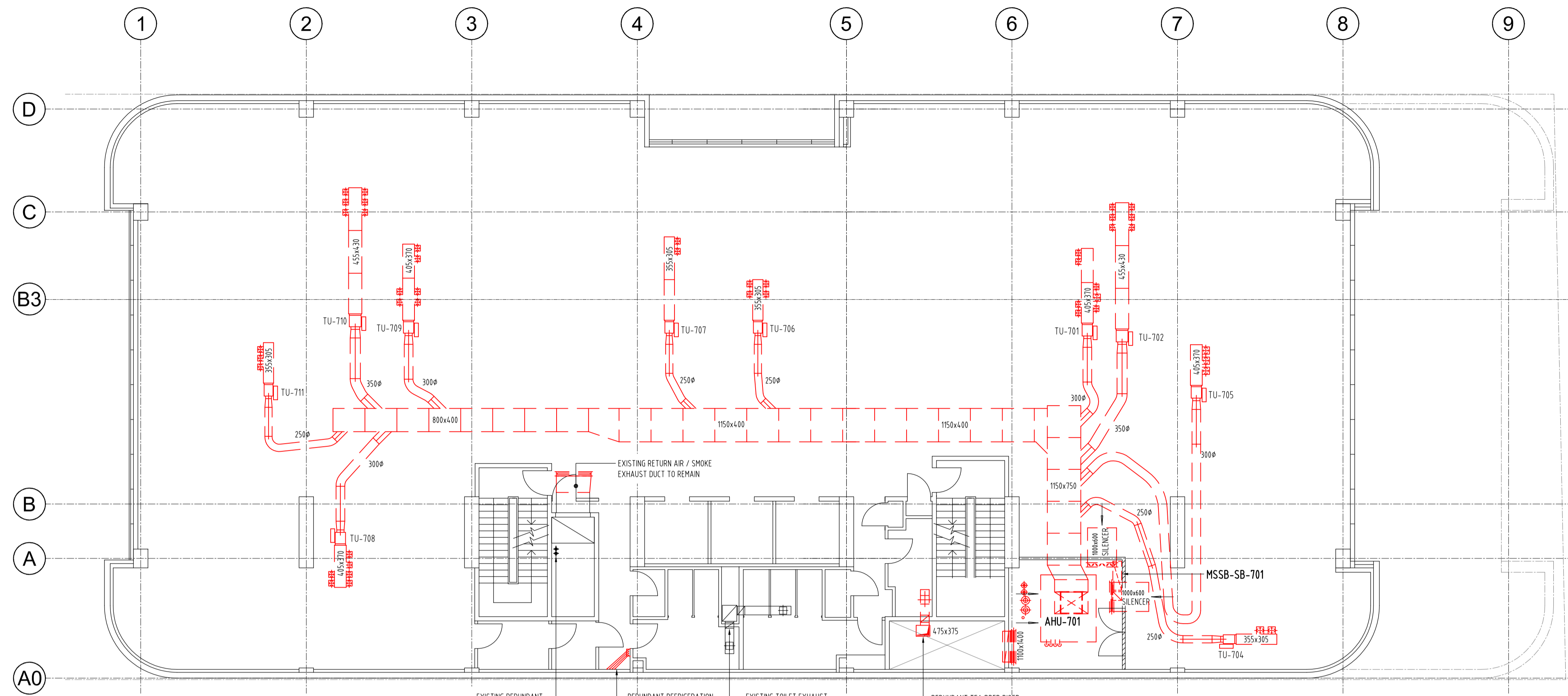
LEVEL 7 - MECHANICAL SERVICES DEMOLITION SCALE 1:100
