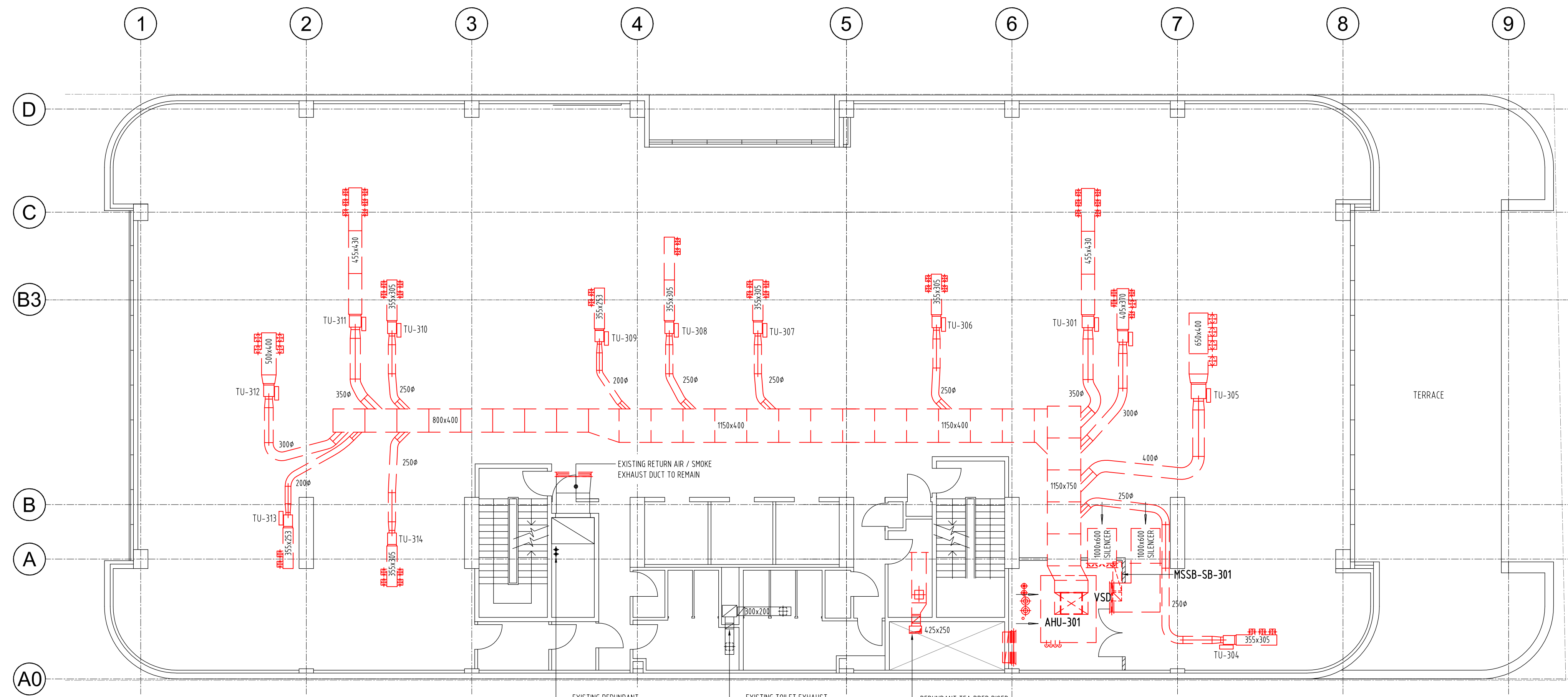
LEVEL 3 - MECHANICAL SERVICES DEMOLITION SCALE 1:100
