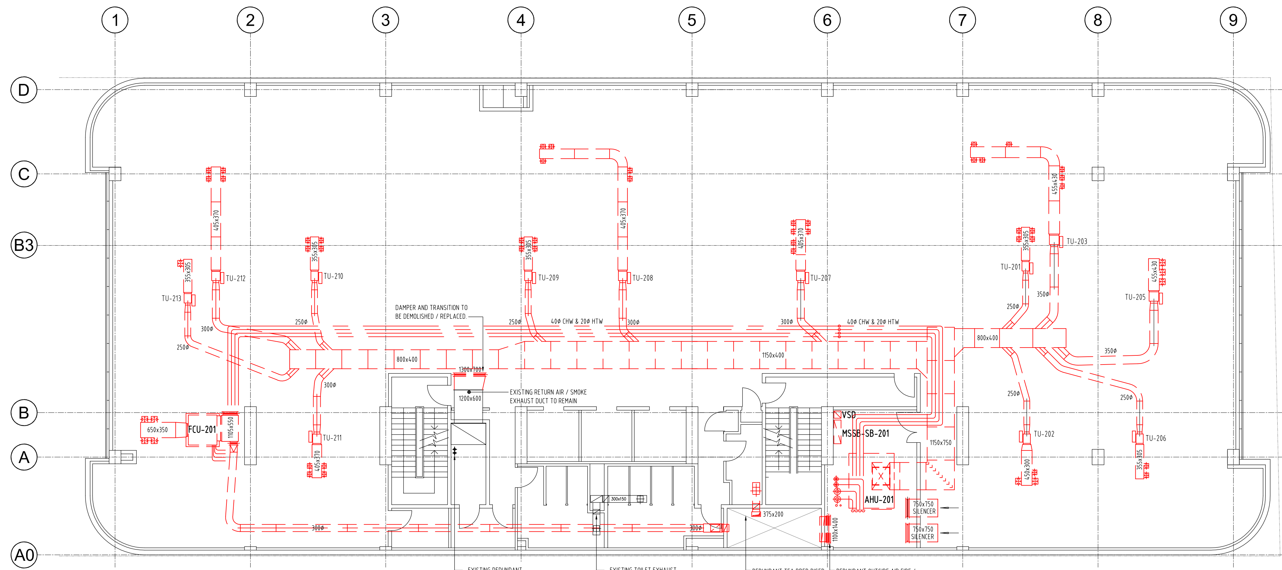
LEVEL 2 - MECHANICAL SERVICES DEMOLITION SCALE 1:100
