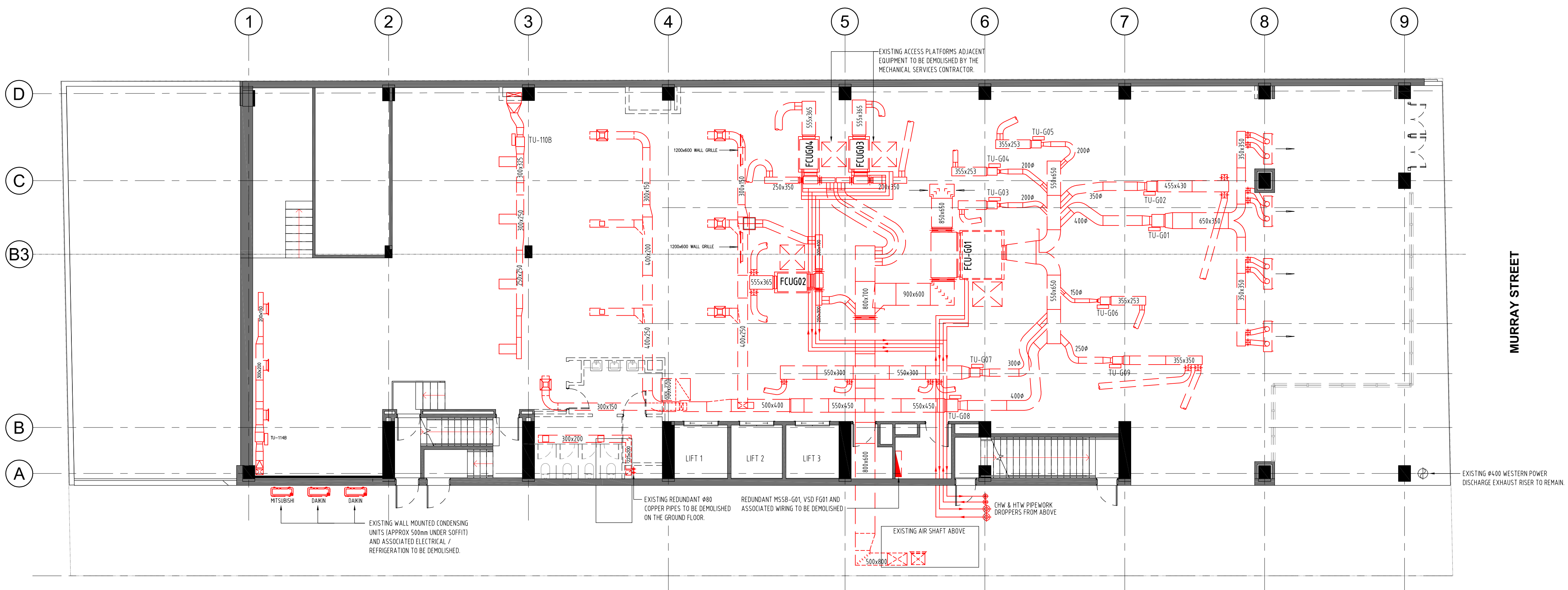
GROUND FLOOR - MECHANICAL SERVICES DEMOLITION SCALE 1:100
