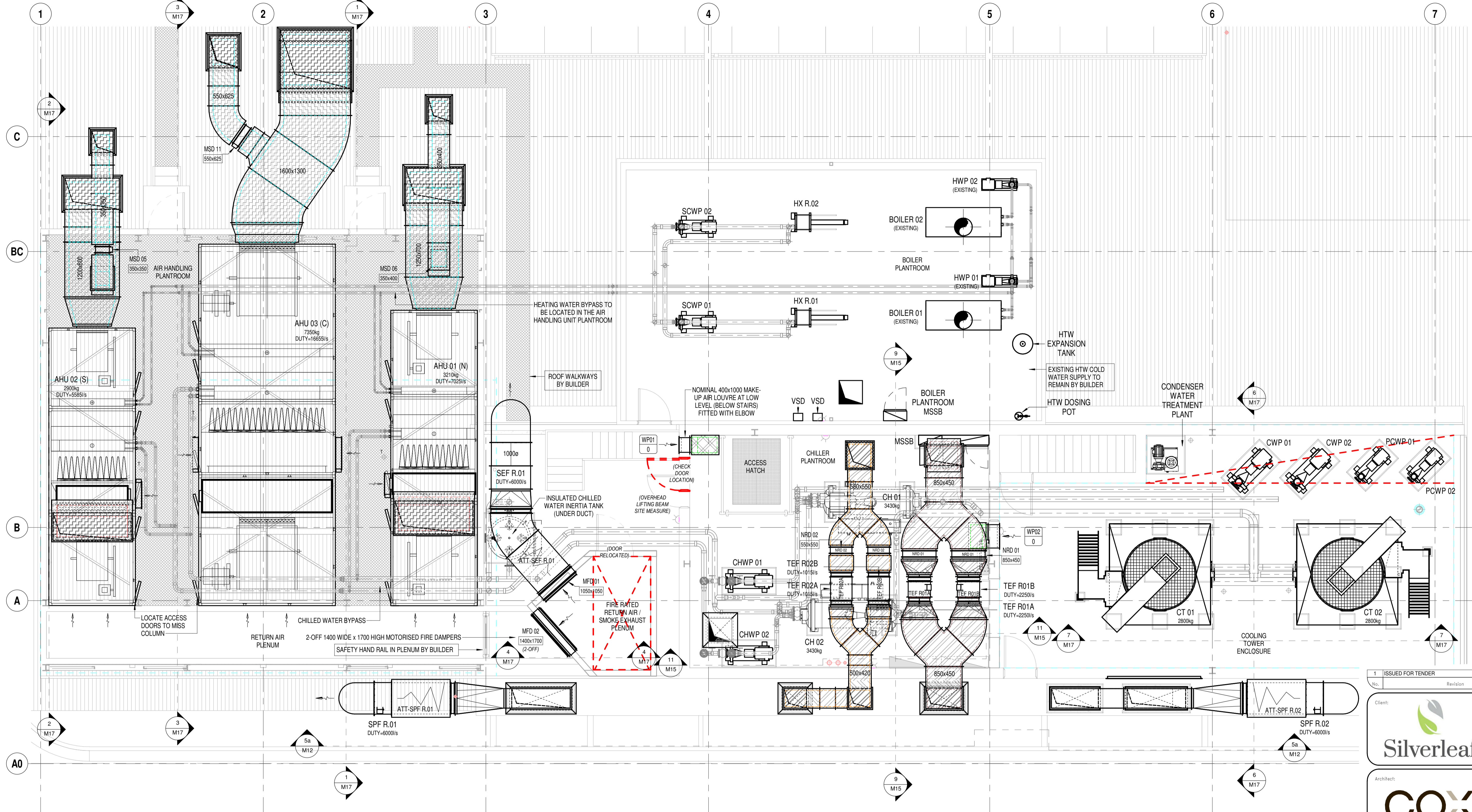
1 ROOF PLANTROOM LAYOUT SCALE 1 : 50
